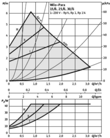
Differenzdruck variabel \Delta p_v
